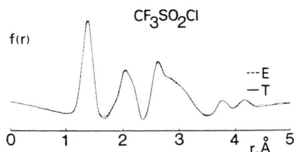
Fig. 2. Experimental (E) and theoretical (T) radial distributions.
